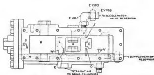
Fig. 2580. Plan of Valve with Cover and Handle Removed.
